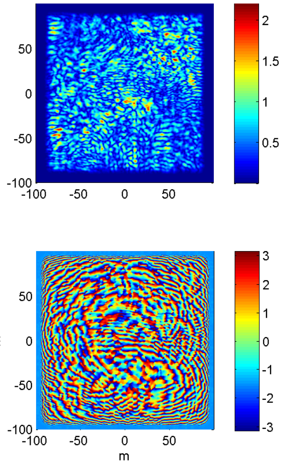
Figure 19. Acoustic amplitude (top) and phase (bottom) for a 10-kHz simulation of a surface reflected field from a bottom-mounted PIES in 3000-m depth water. 2048 x 2048 domain.
