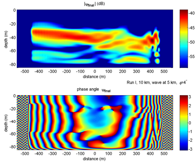
Figure 9. Intensity and phase are shown for a situation similar to that of the previous figure, except the wave angle is \phi = 4^\circ . This situation shows horizontal refraction of the sound. The depth-averaged sound intensity is not symmetric around y = 0 , unlike the \phi = 16^\circ case (not shown). The phase minimum is not at y = 0 .
