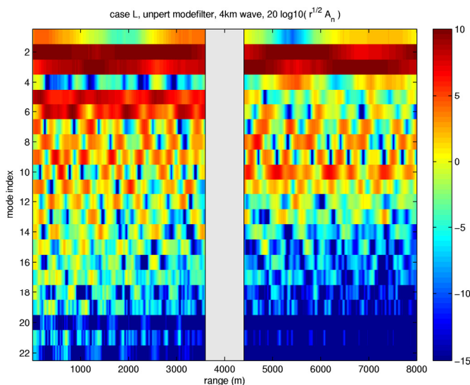
Figure 15. The magnitudes of mode coefficients times range^{1/2} are computed along y = 0 for a case similar to those shown earlier (400 Hz, source depth 40 m, one 10:95 nonlinear internal wave). The internal wave is at angle 30.4^\circ with position x = 4000 m at y = 0 . Mode filtering is performed with mode functions (computed using the code FEMODE.F from Naval Research Lab.) for the unperturbed environment, i.e. outside the wave. The area within the wave where these are not the correct mode functions is shown in gray. Modes should be uncoupled outside the wave, so the oscillations in range of the coefficients show small numerical errors known to be associated with overly long range step increment. Despite this, mode coupling in the wave, which is expected, can be seen to strip energy from modes 5 and 6.
